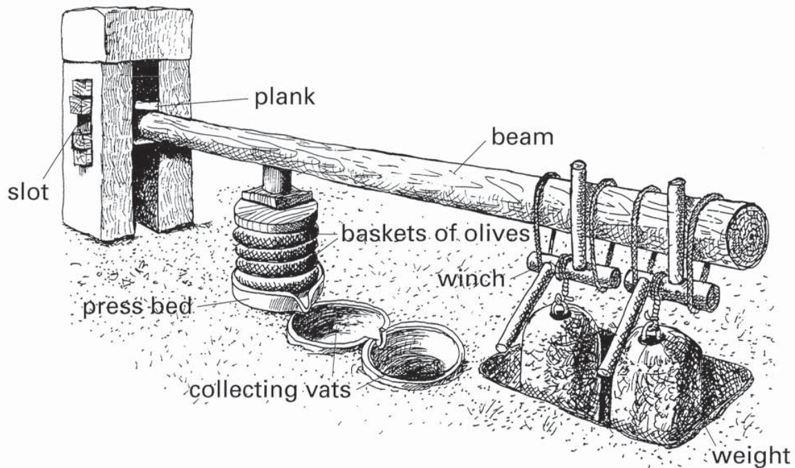
FIG. 2. An ancient lever-and-weights oil press excavated at Khirbet Zibdi, Israel. The oil was separated from the heavier lees when the oil flowed from the first collecting vat to the second. Drawing by Shlomo Sawady; text added. Courtesy Eretz Israel Museum, Tel Aviv, Israel. From Rafael Frankel, Shmuel Avitsur, and Etan Ayalon, History and Technology of Olive Oil in the Holy Land (Arlington, Va.: Olearius Editions; Tel Aviv: Eretz Israel Museum, 1994), 41.
